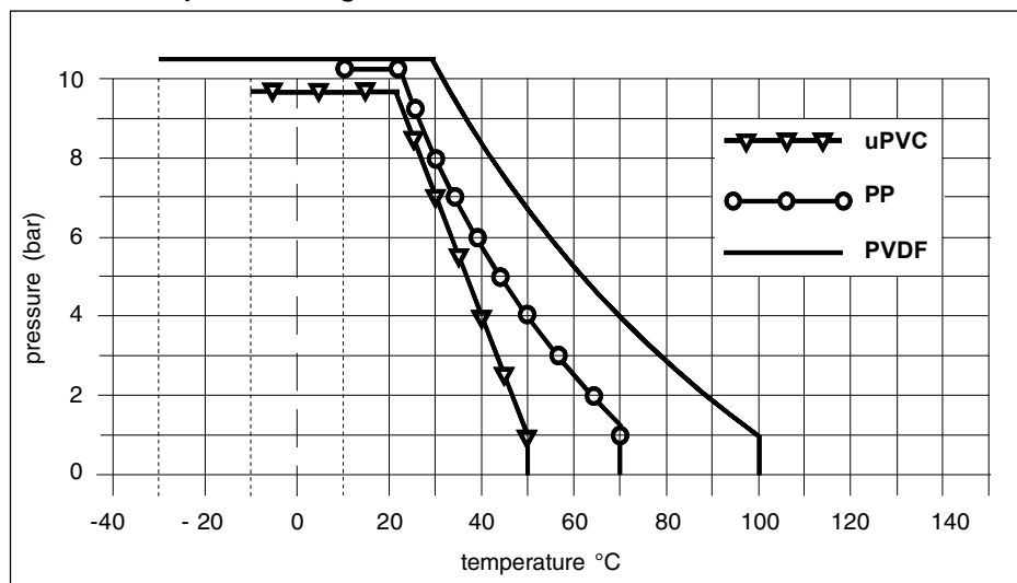
Pressure-temperature diagram
